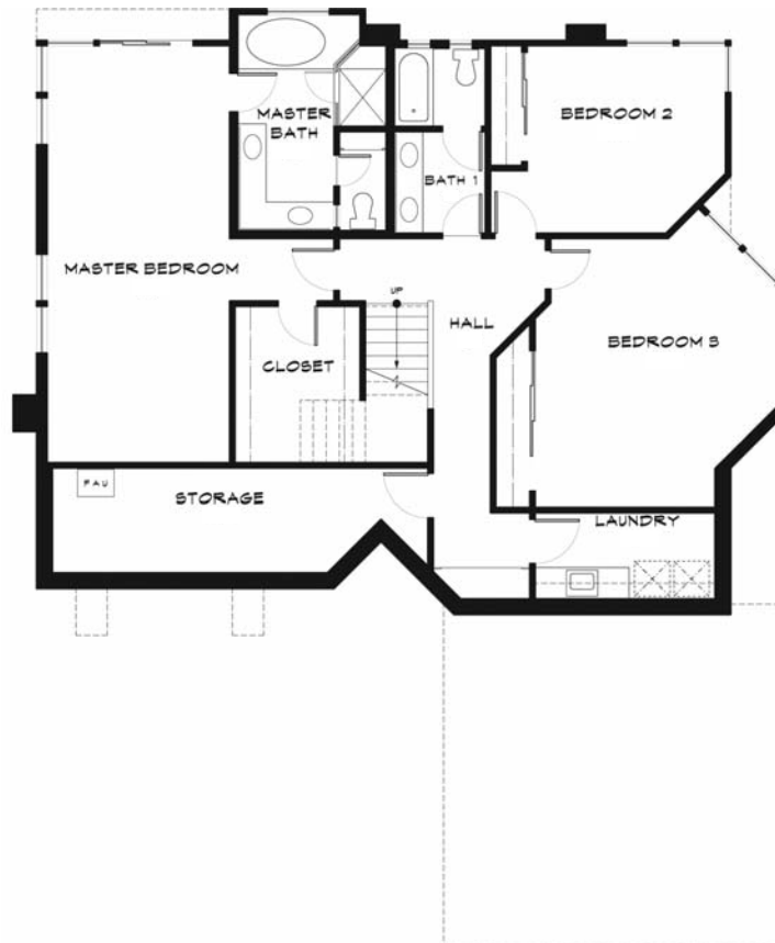
Lower Level
